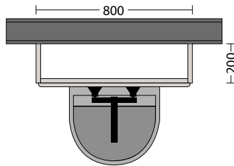
Standard Pre Assembled Boxed Unit
