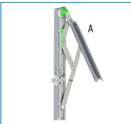
Vela top opening Hinge with Automatic Safety Catch
