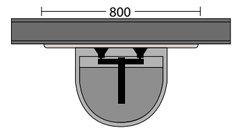
Standard Pre Assembled Recessed Unit
