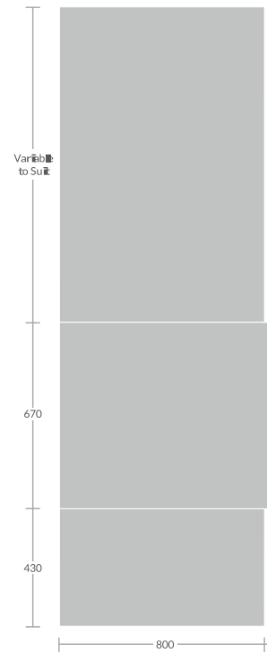
Standard Pre Assembled Recessed Unit
