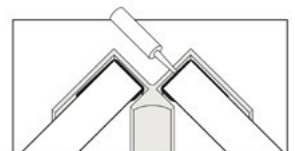
Showerwall Internal Trim
